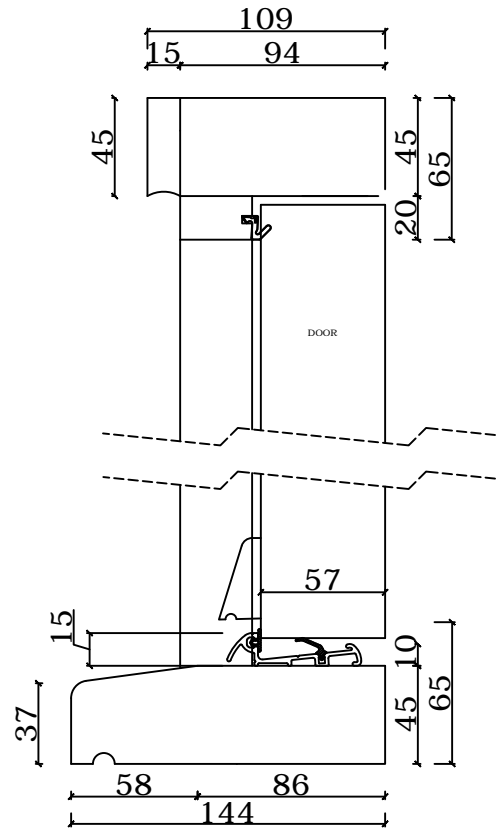
Standard door and sill inward opening
