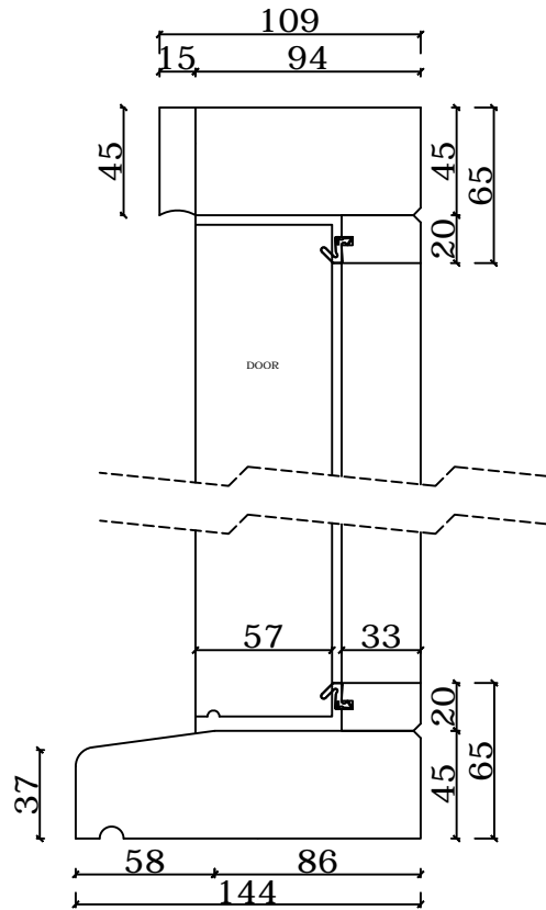
Standard door and sill outward opening
